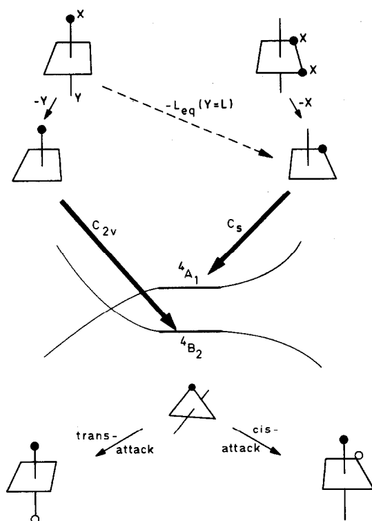
Fig. 6. Pattern of photosubstitutions in mono- and disubstituted chromium(III) complexes, as predicted from the three stereochemical rules. X is assumed to be a weak-field ligand. The relevant part of the correlation diagram for the association reactions of the TBP is included. Three possible reactions are envisaged: (i) Y loss from an axially labilized \text{trans-CrL}_4\text{XY} leads to a \text{cis-CrL}_4\text{XS} product via a C_{2v} path; (ii) X loss from equatorially labilized \text{cis-CrL}_4\text{X}_2 gives rise to a \text{trans} product via a C_5 path. (iii) The dashed line represents subsidiary equatorial L loss from the predominantly axially labilized complex in its {}^4E_g excited state. In case Y = L , this pathway leads to the same SPY intermediate as considered sub (ii), and ultimately to the same photoproducts.
